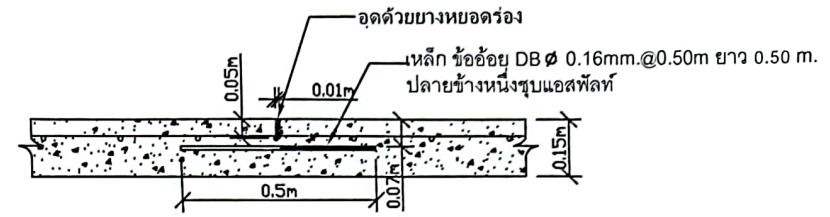
CONTRACTION JOIN
