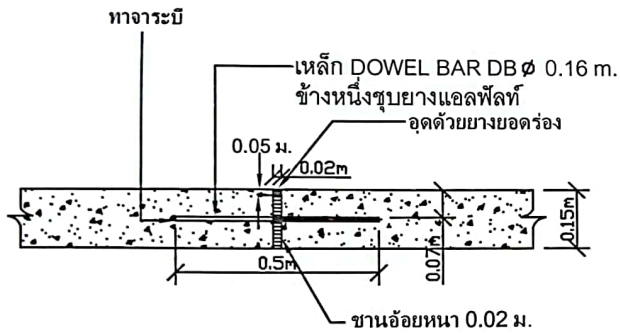
EXPANSION JOINT
